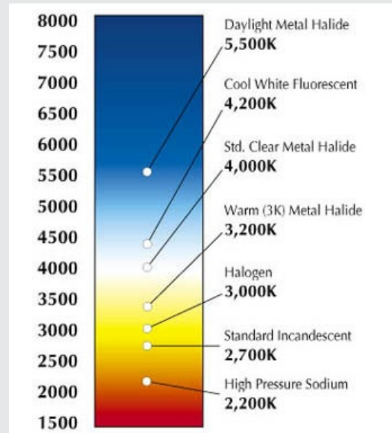
Figure 17 – Colour temperature
